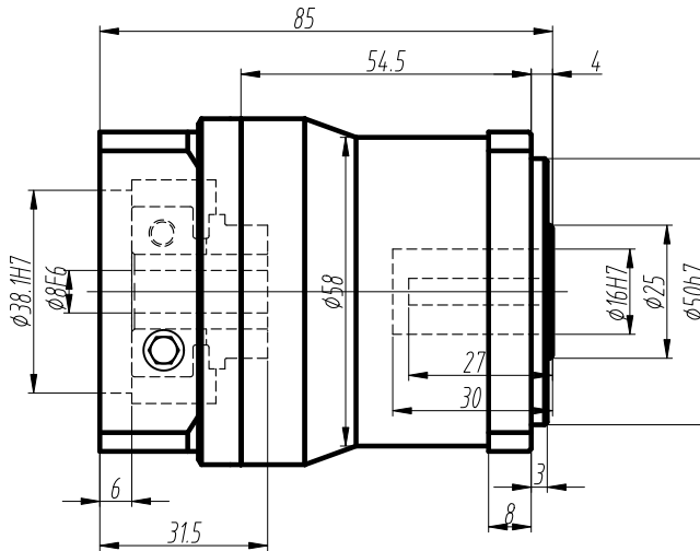
标准轴 Standard output shaft
